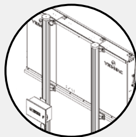
Z-Bar mounting for bridge, gantry i-beam posts structures
